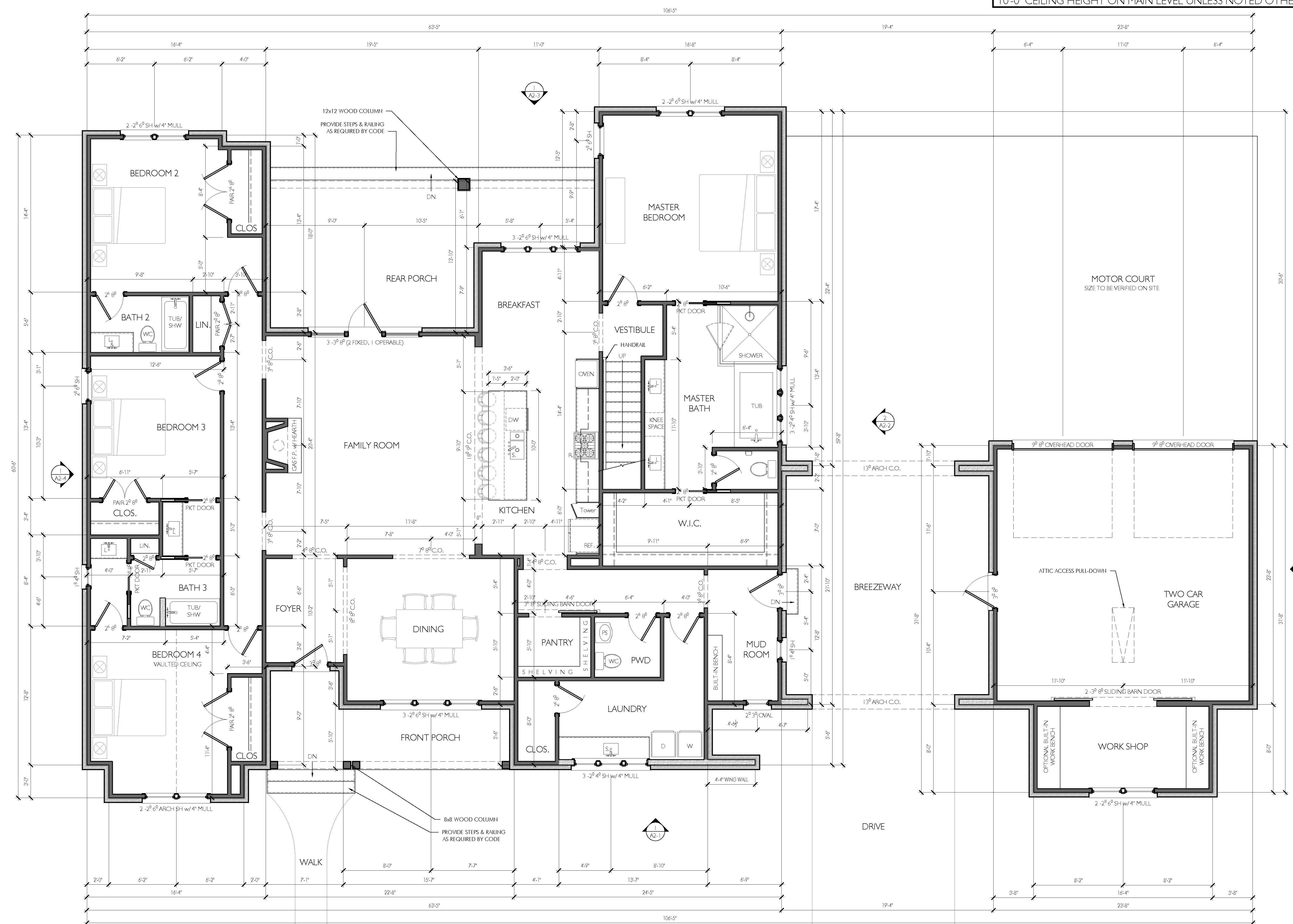
1 MAIN LEVEL FLOOR PLAN 1/4" = 1'-0"
